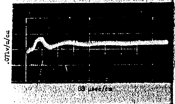
Fig. 3.92 Broadband pulse Shot No. 2 3400 km from ground zero
